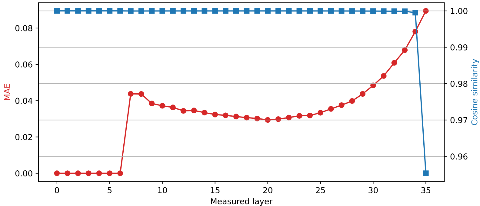
SmolLM3-3B | Quantized layer 6 | float64 → int4
