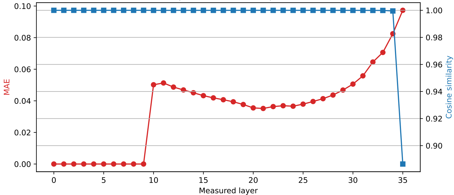
SmolLM3-3B | Quantized layer 9 | float64 \rightarrow int4
