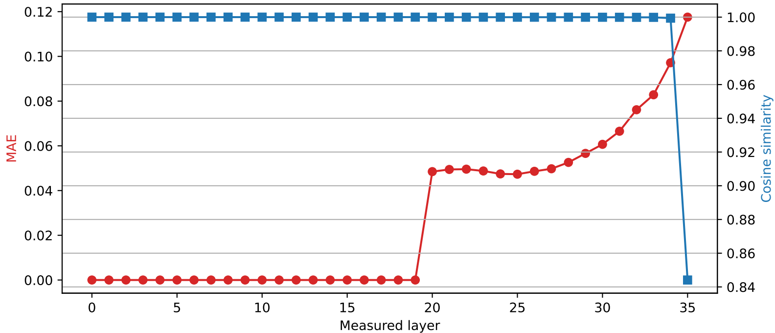
SmolLM3-3B | Quantized layer 19 | float64 → int4
