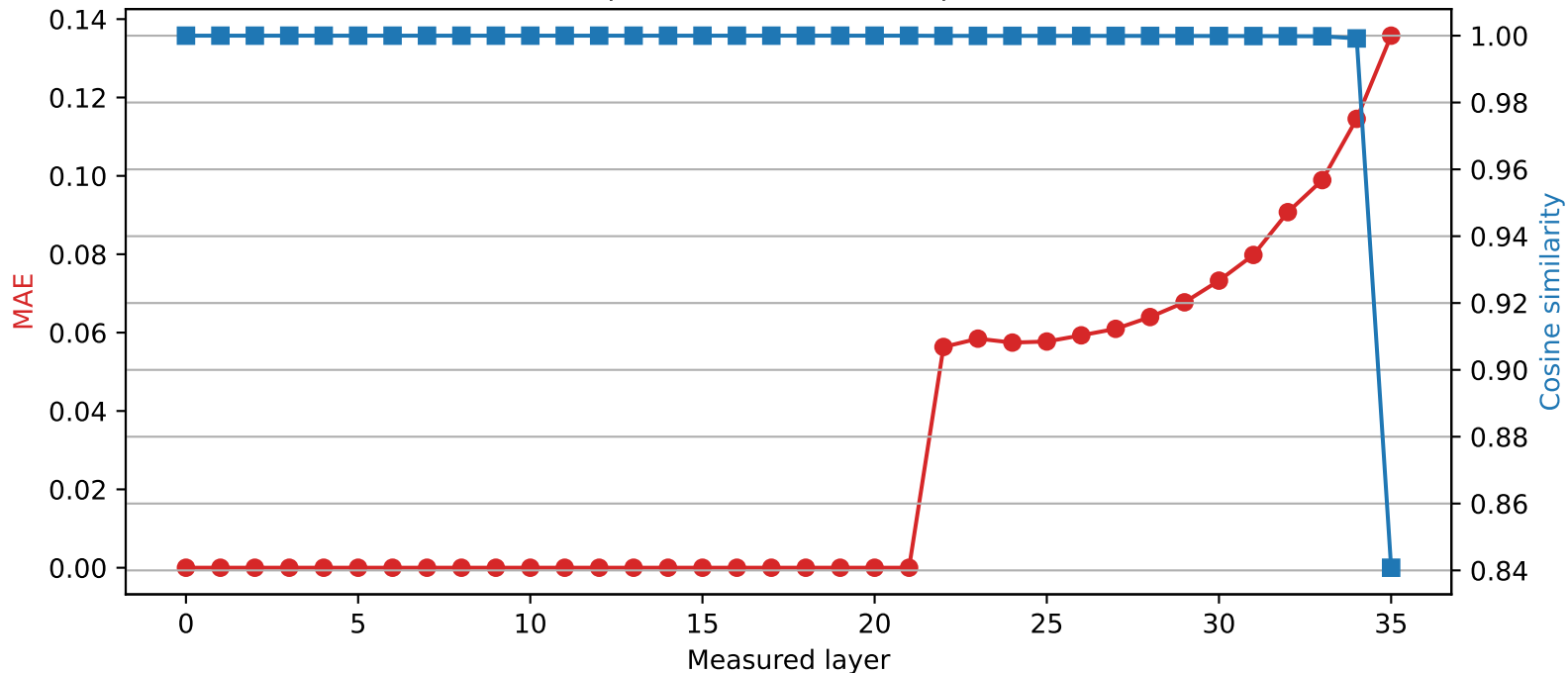
SmolLM3-3B | Quantized layer 21 | float64 → int4
