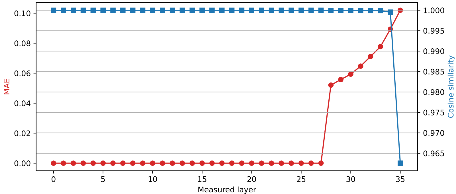
SmolLM3-3B | Quantized layer 27 | float64 \rightarrow int4
