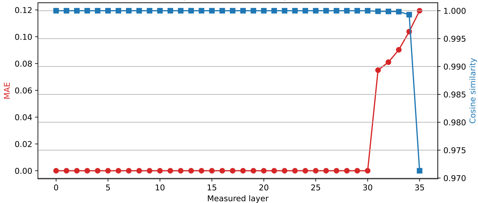
SmolLM3-3B | Quantized layer 30 | float64 → int4
