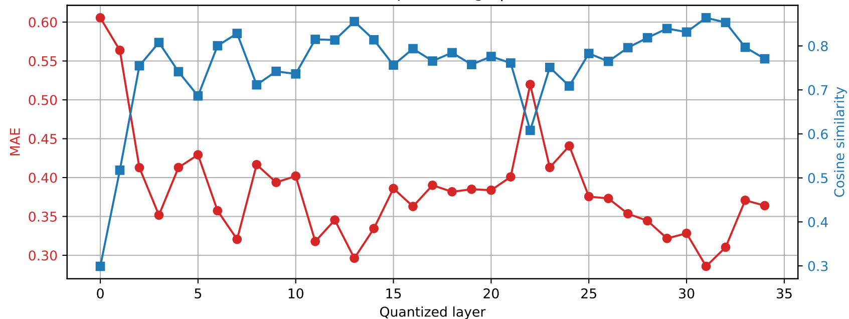
SmolLM3-3B | Prompt 1 Final RMSNorm output damage | float64 \rightarrow int4
