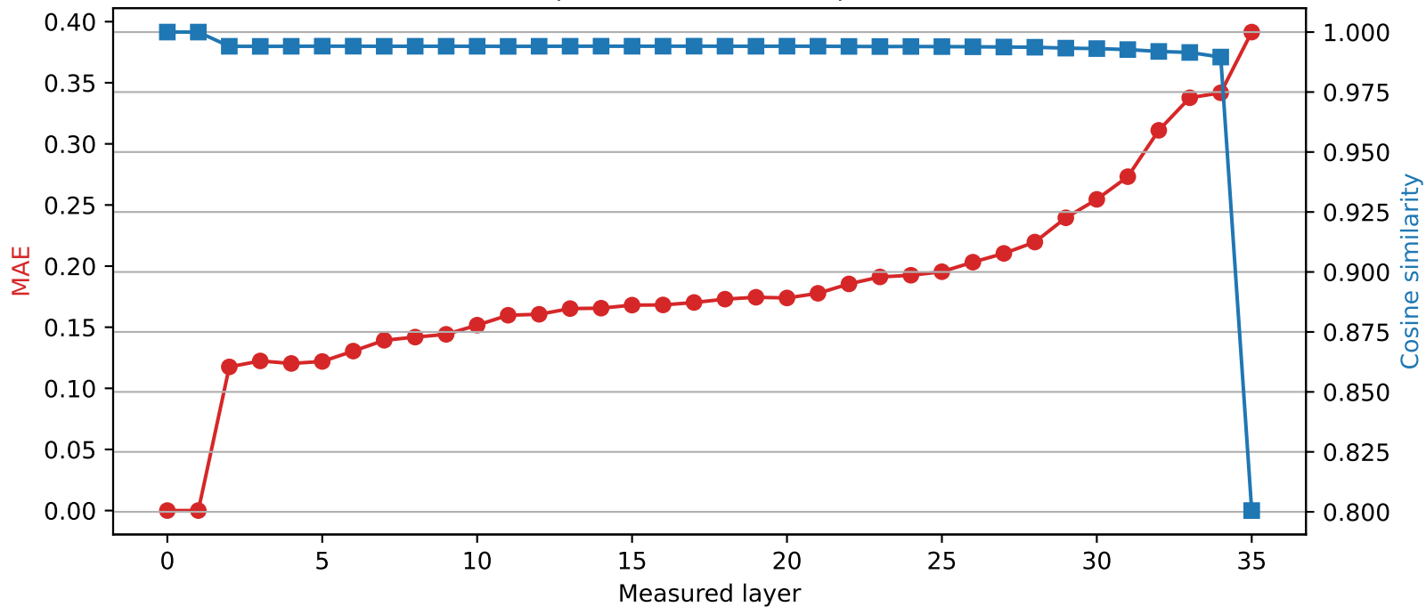
SmolLM3-3B | Quantized layer 1 | float64 → int4
