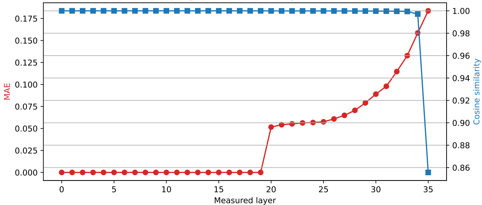
SmolLM3-3B | Quantized layer 19 | float64 \rightarrow int4
