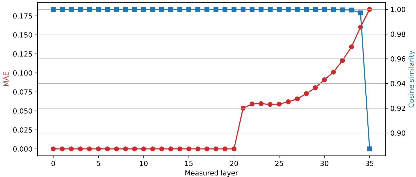
SmolLM3-3B | Quantized layer 20 | float64 \rightarrow int4
