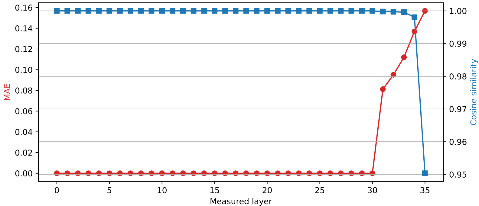
SmolLM3-3B | Quantized layer 30 | float64 \rightarrow int4
