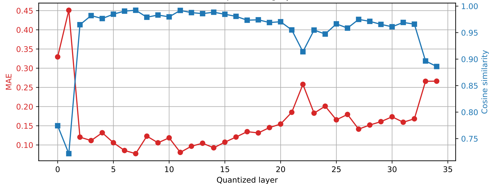
SmolLM3-3B | Prompt 2 Final RMSNorm output damage | float64 → int4
