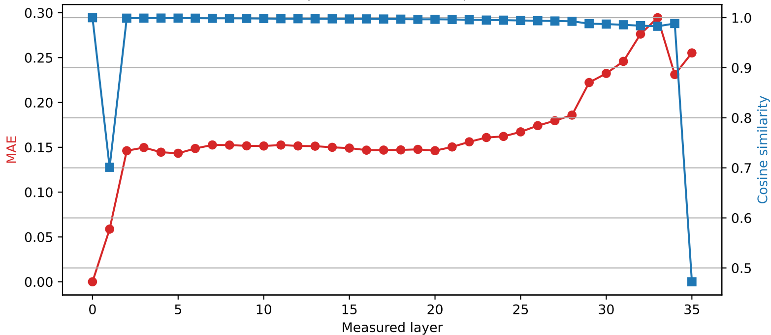
SmolLM3-3B | Quantized layer 0 | float64 \rightarrow int4
