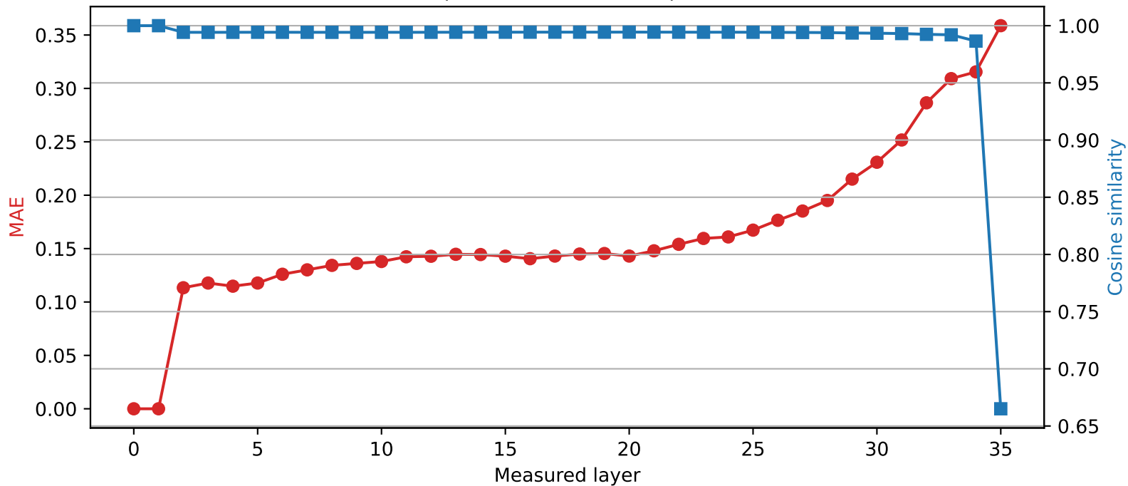
SmolLM3-3B | Quantized layer 1 | float64 \rightarrow int4
