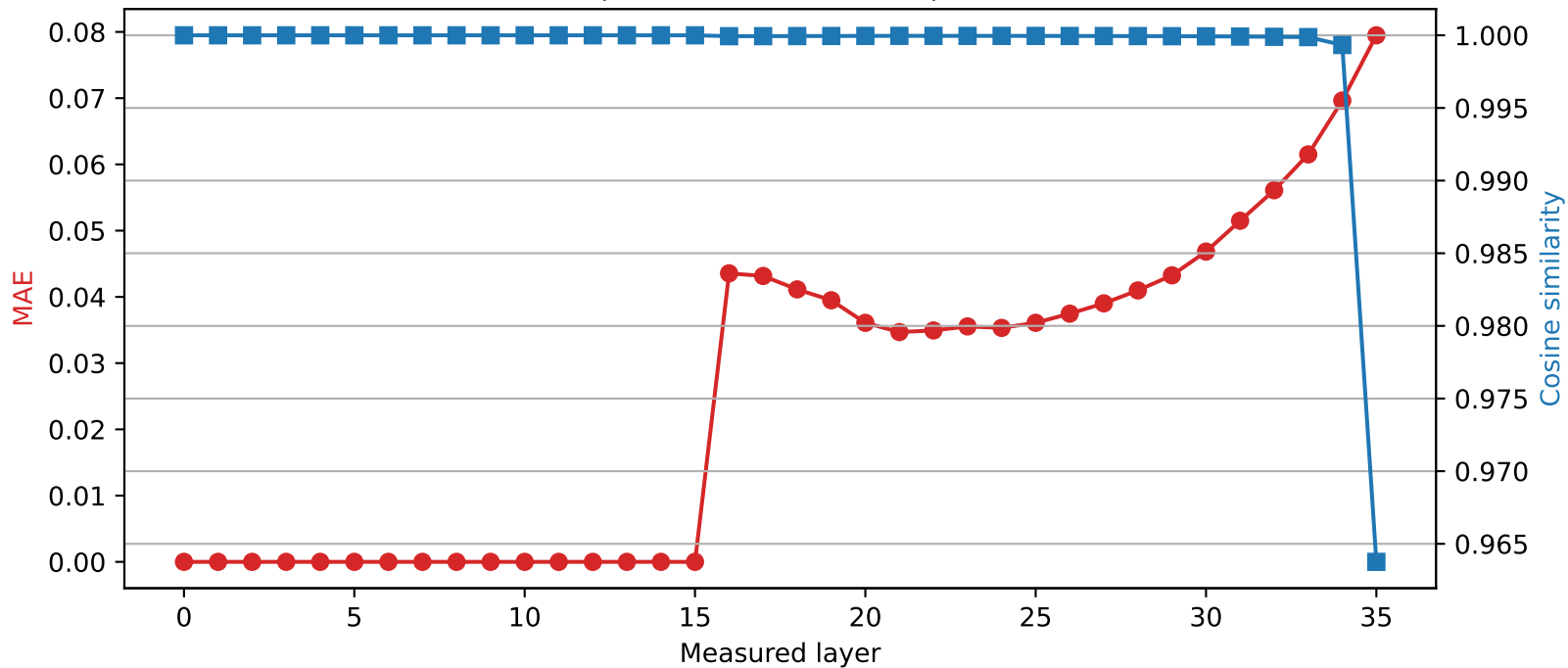
SmolLM3-3B | Quantized layer 15 | float64 → int4
