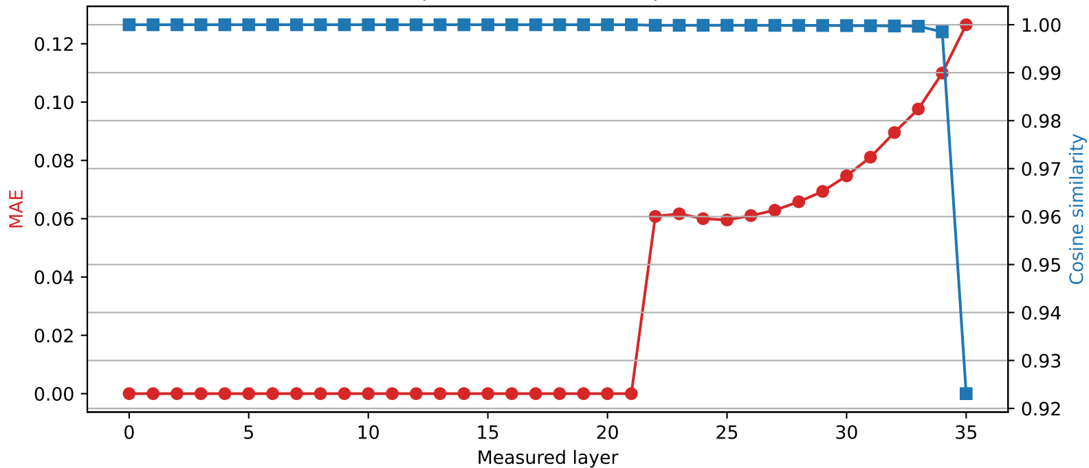
SmolLM3-3B | Quantized layer 21 | float64 \rightarrow int4
