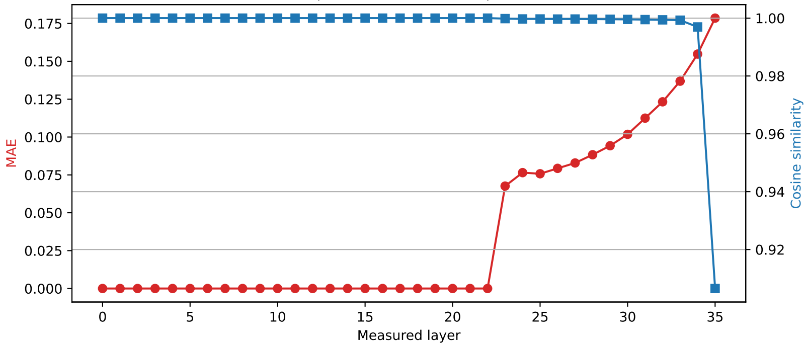
SmolLM3-3B | Quantized layer 22 | float64 → int4
