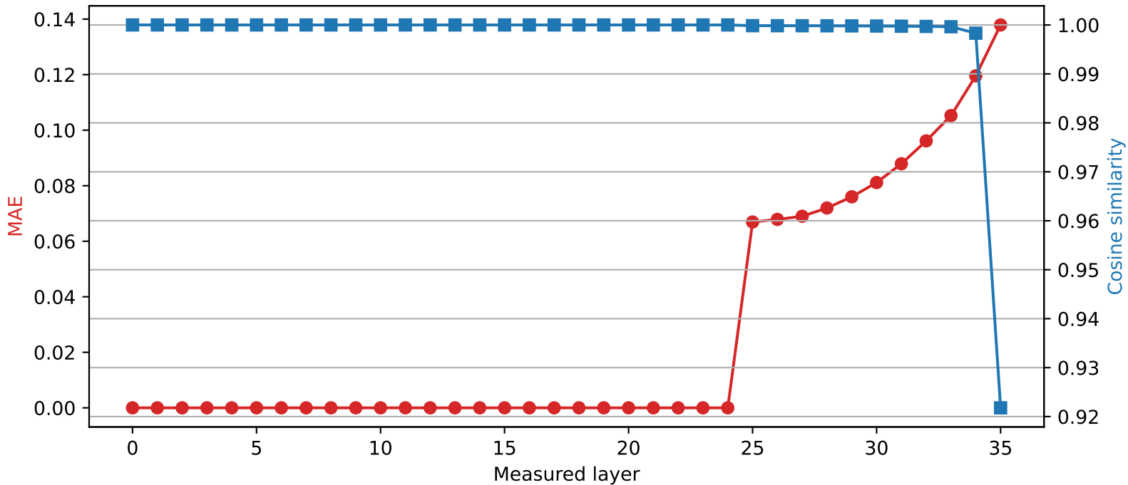
SmolLM3-3B | Quantized layer 24 | float64 → int4
