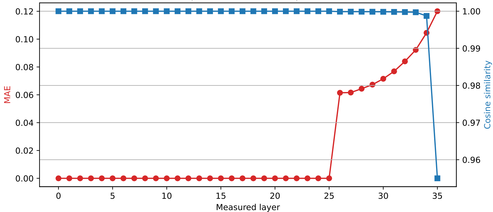
SmolLM3-3B | Quantized layer 25 | float64 \rightarrow int4
