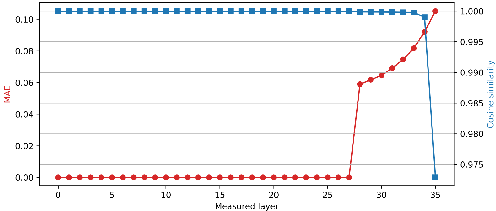
SmolLM3-3B | Quantized layer 27 | float64 → int4
