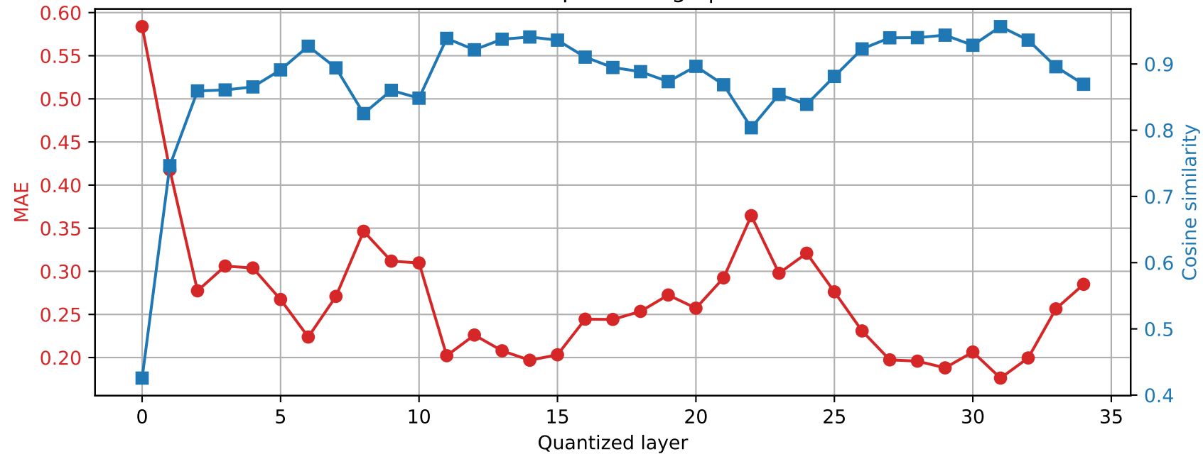
SmolLM3-3B | Prompt 3 Final RMSNorm output damage | float64 \rightarrow int4
