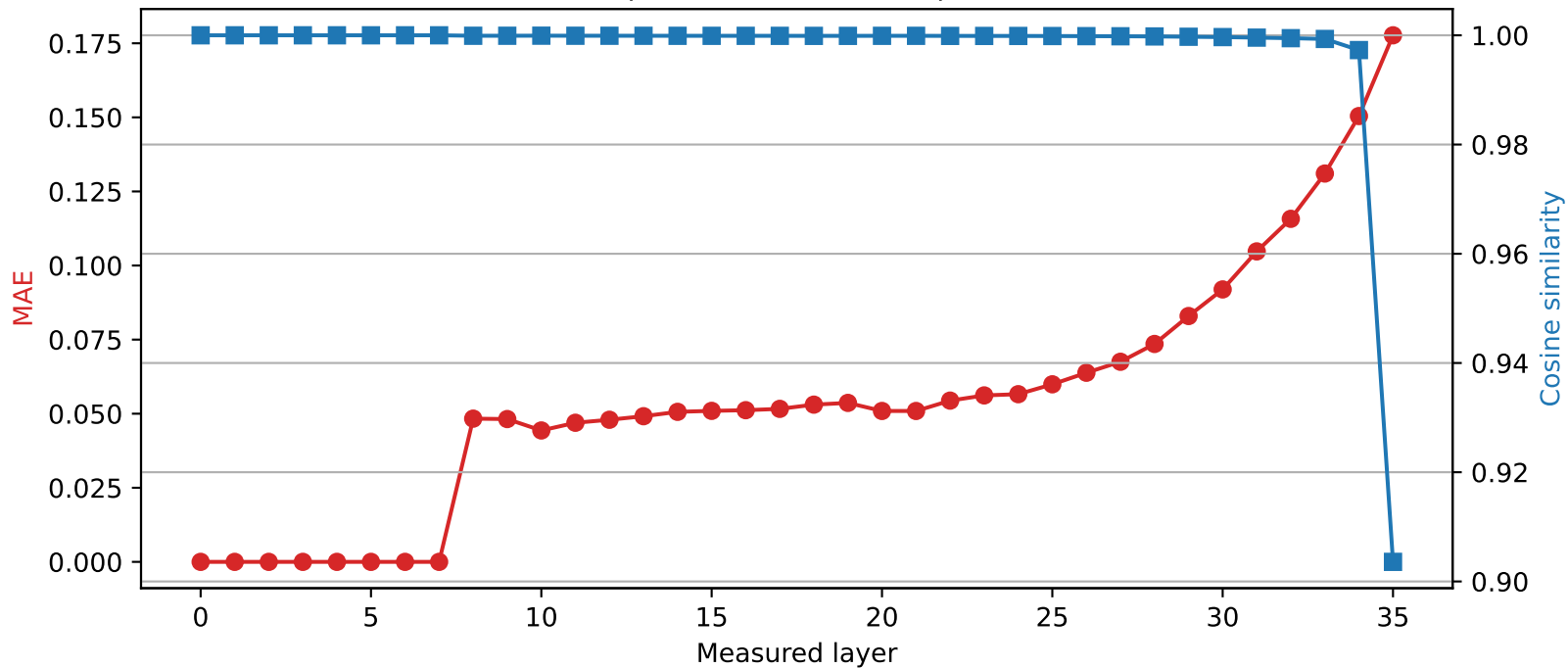
SmolLM3-3B | Quantized layer 7 | float64 \rightarrow int4
