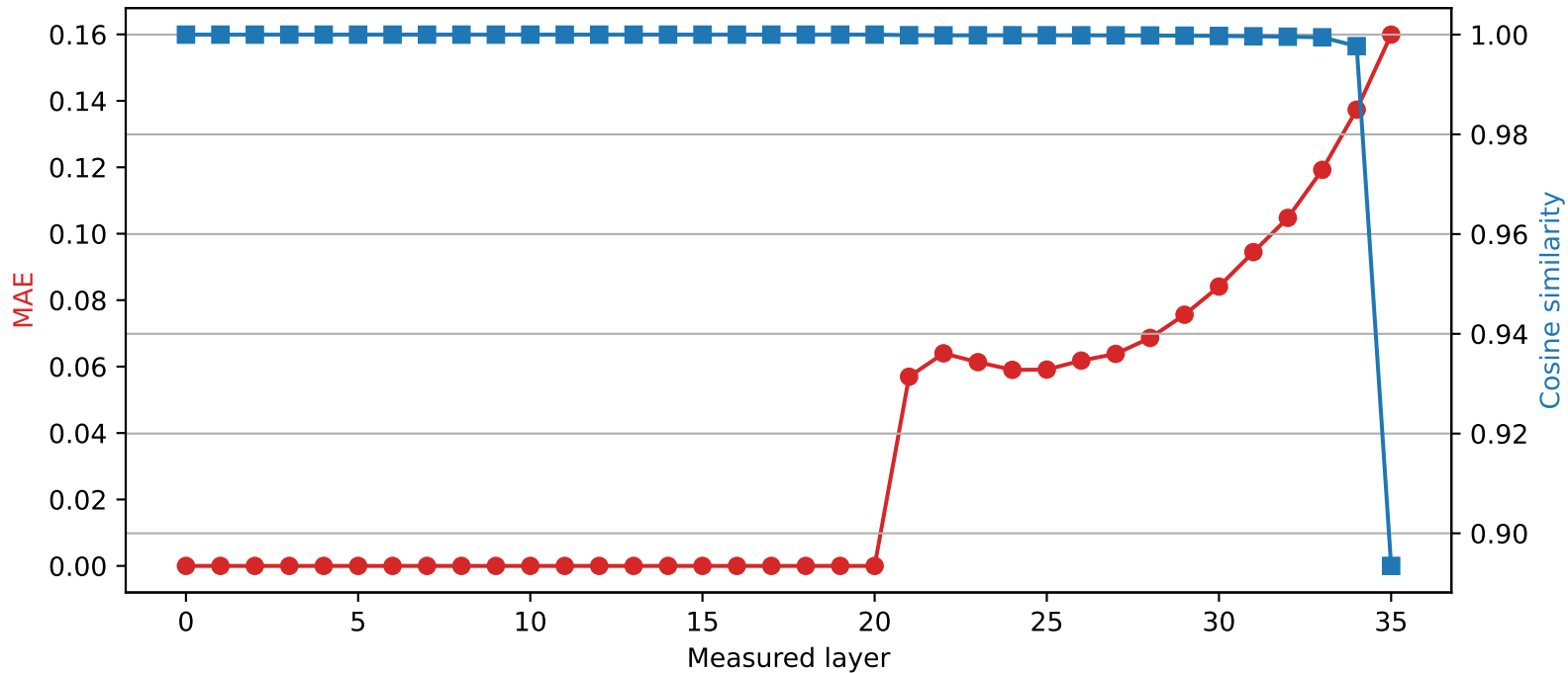
SmolLM3-3B | Quantized layer 20 | float64 → int4
