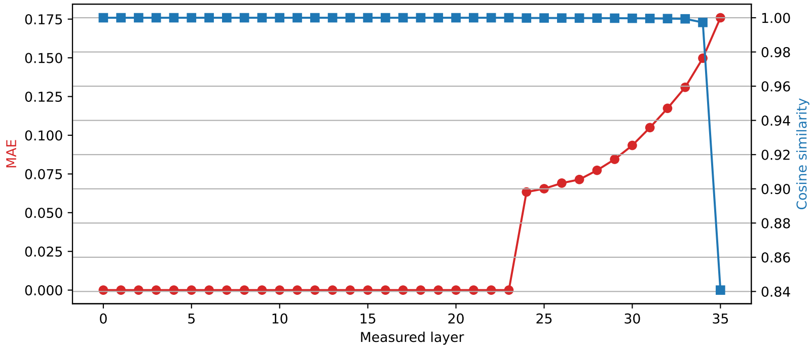
SmolLM3-3B | Quantized layer 23 | float64 → int4
