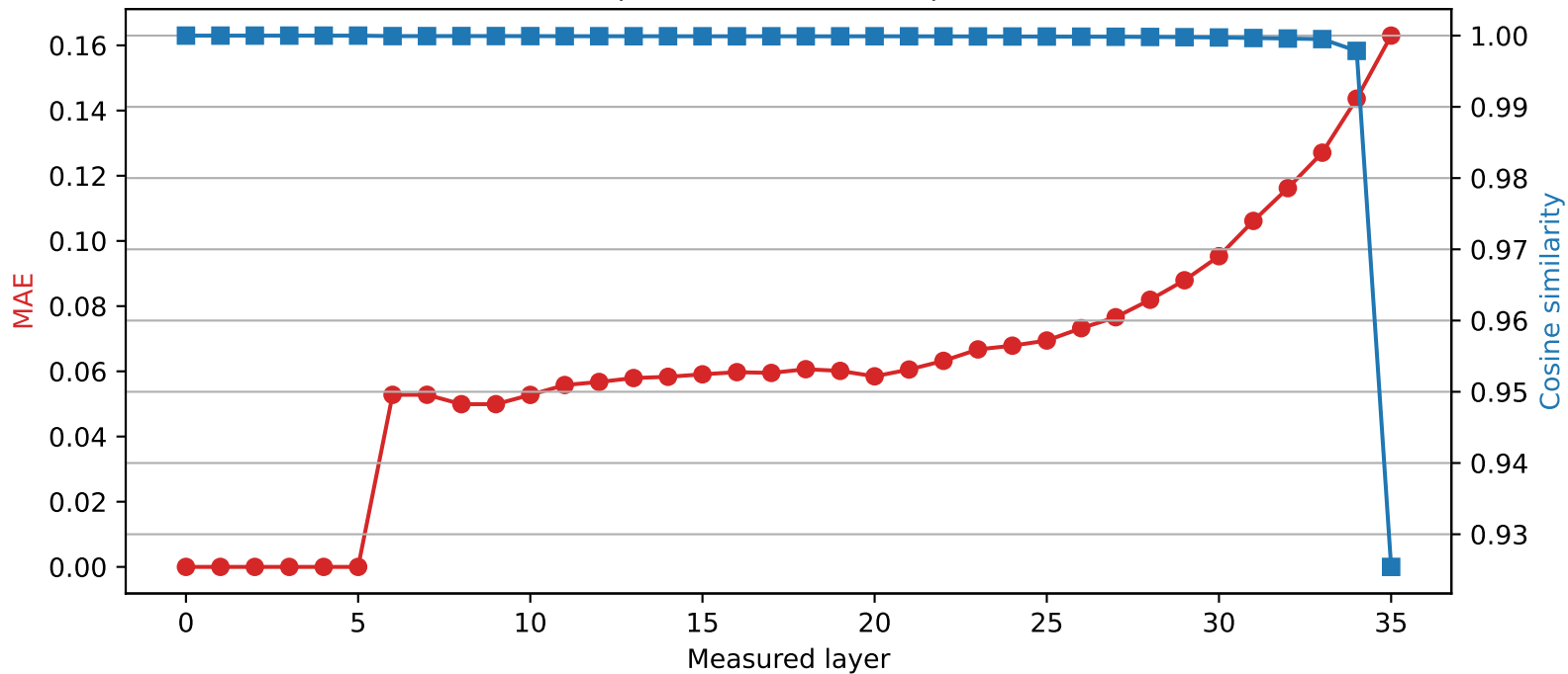
SmolLM3-3B | Quantized layer 5 | float64 \rightarrow int4
