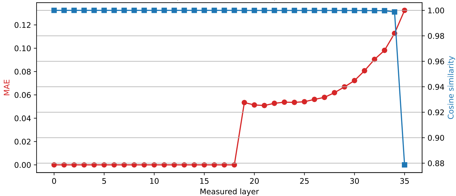
SmolLM3-3B | Quantized layer 18 | float64 → int4
