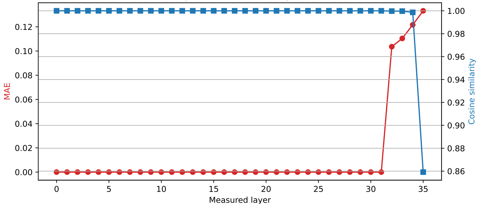
SmolLM3-3B | Quantized layer 31 | float64 → int4
