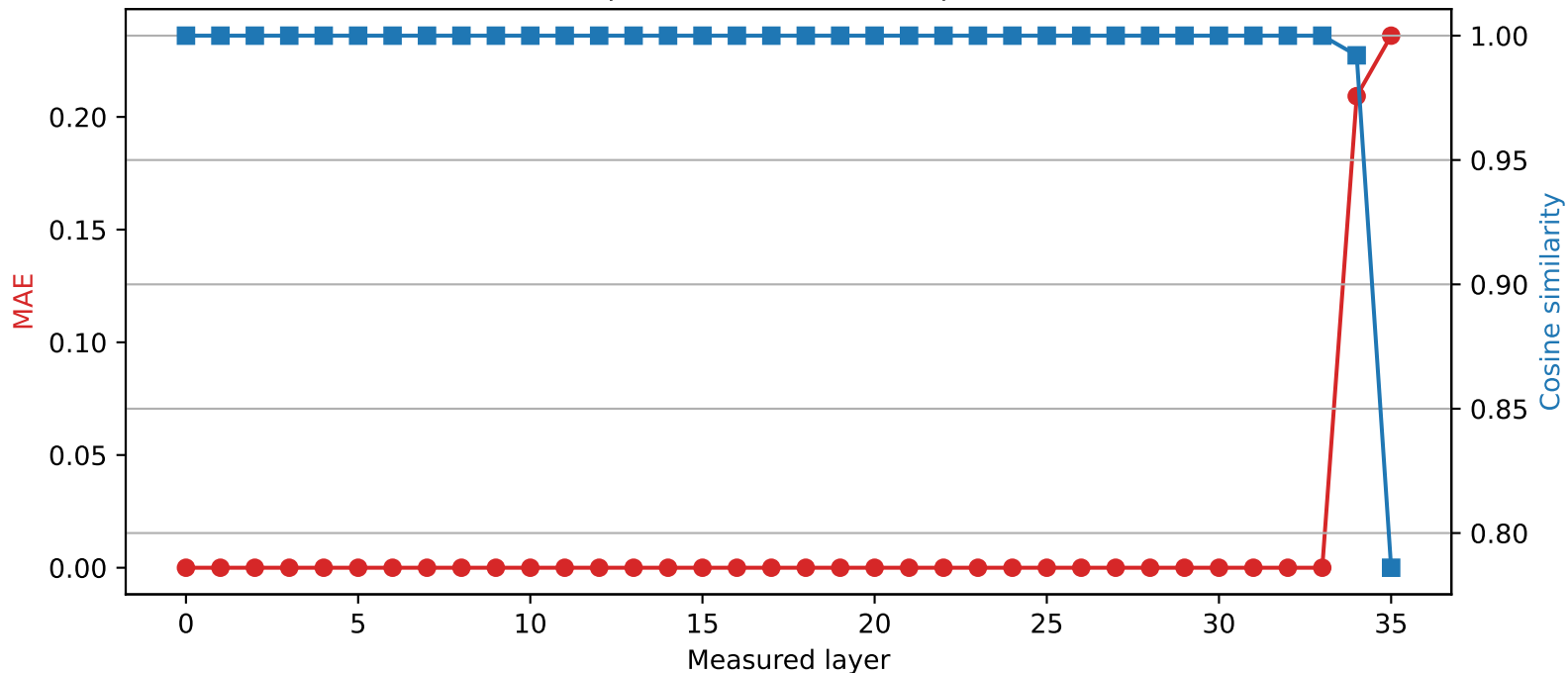
SmolLM3-3B | Quantized layer 33 | float64 \rightarrow int4
