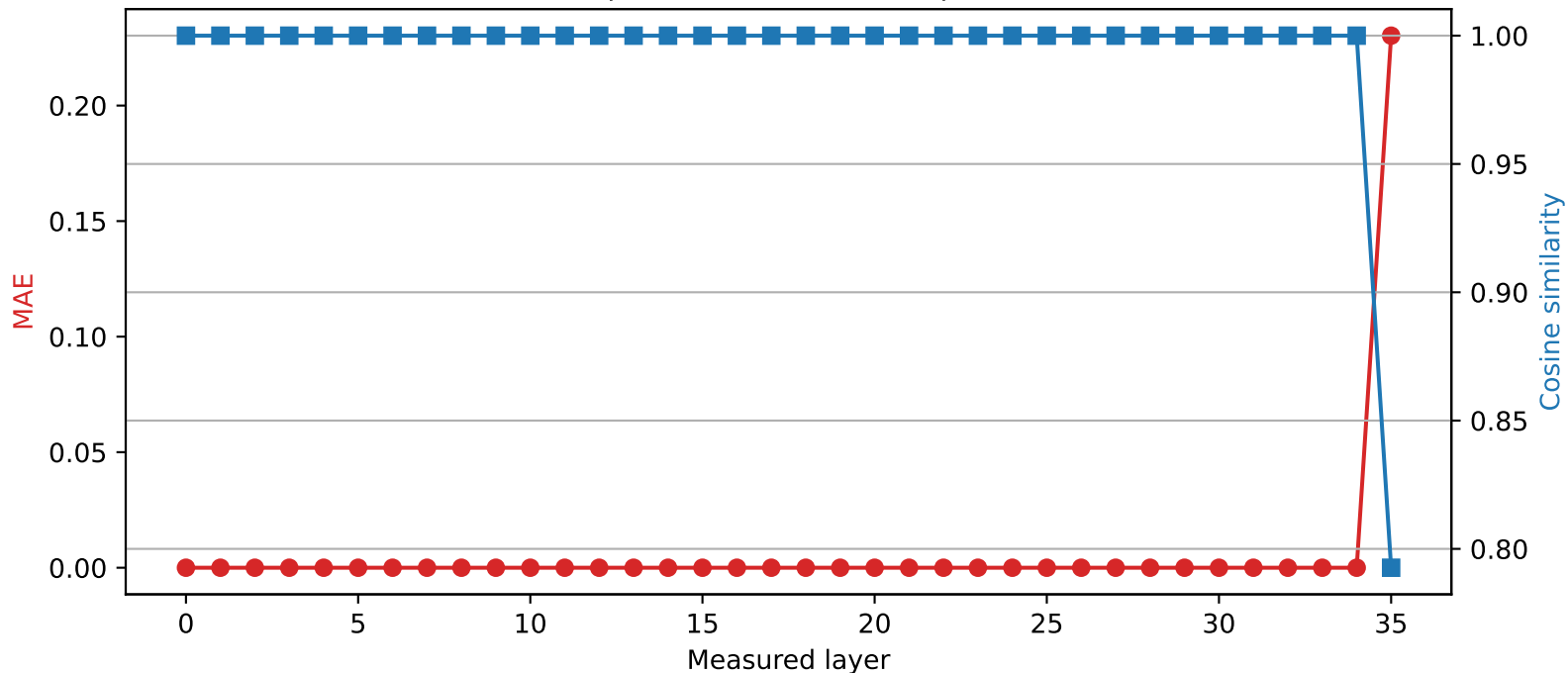
SmolLM3-3B | Quantized layer 34 | float64 \rightarrow int4
