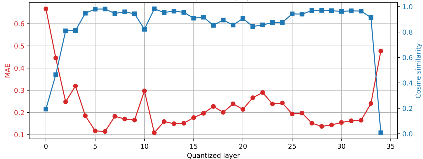
SmolLM3-3B | Prompt 0 Final RMSNorm output damage | float64 \rightarrow int2
