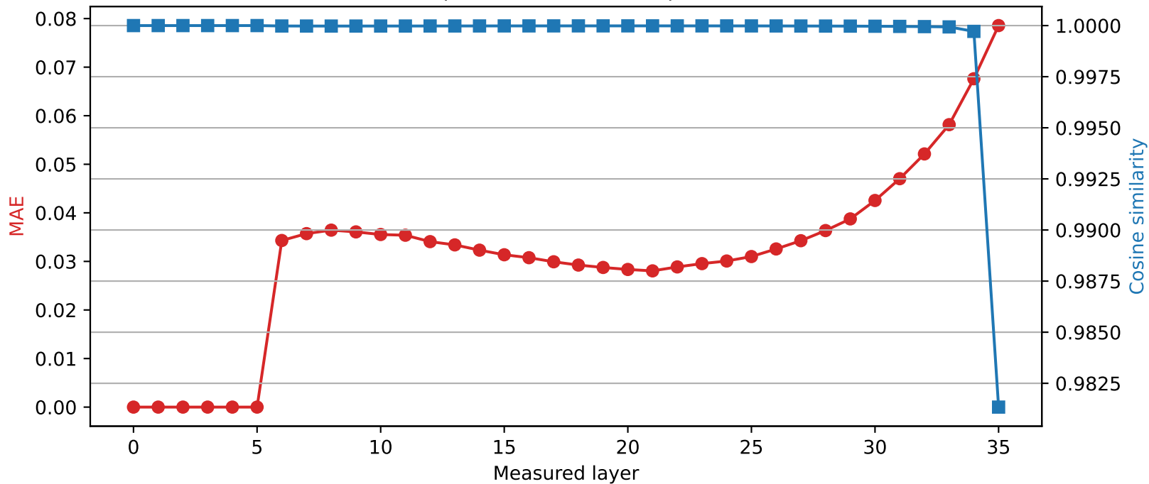
SmolLM3-3B | Quantized layer 5 | float64 \rightarrow int2
