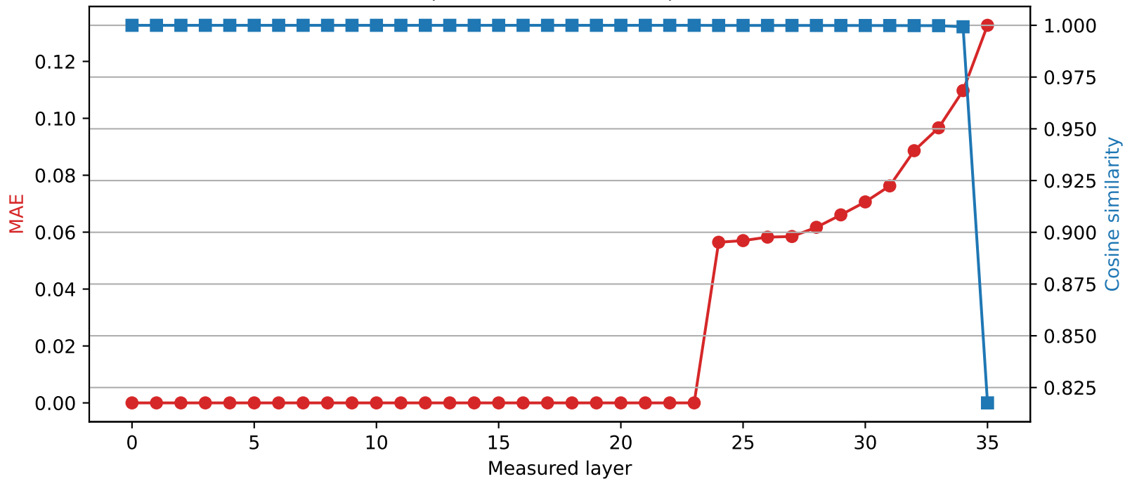
SmolLM3-3B | Quantized layer 23 | float64 → int2
