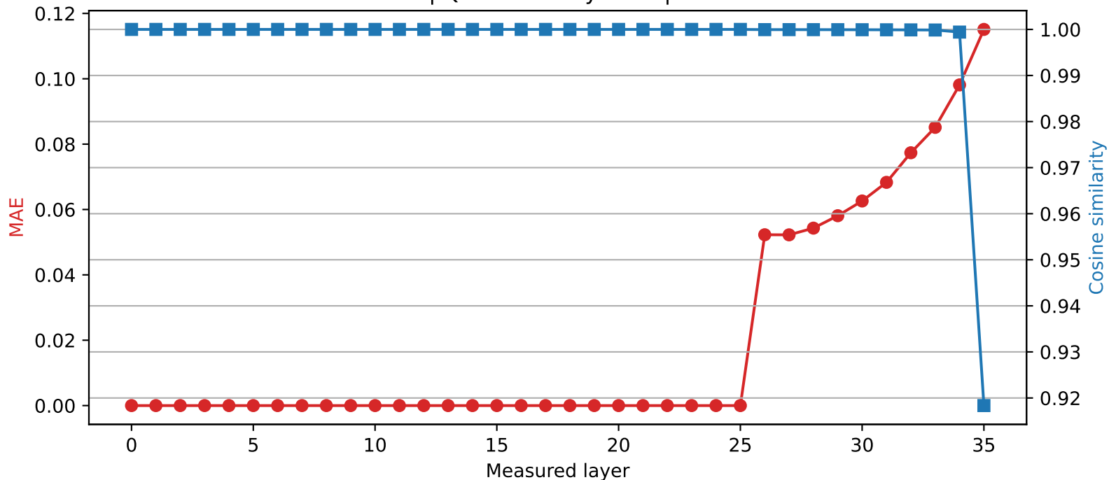
SmolLM3-3B | Quantized layer 25 | float64 → int2
