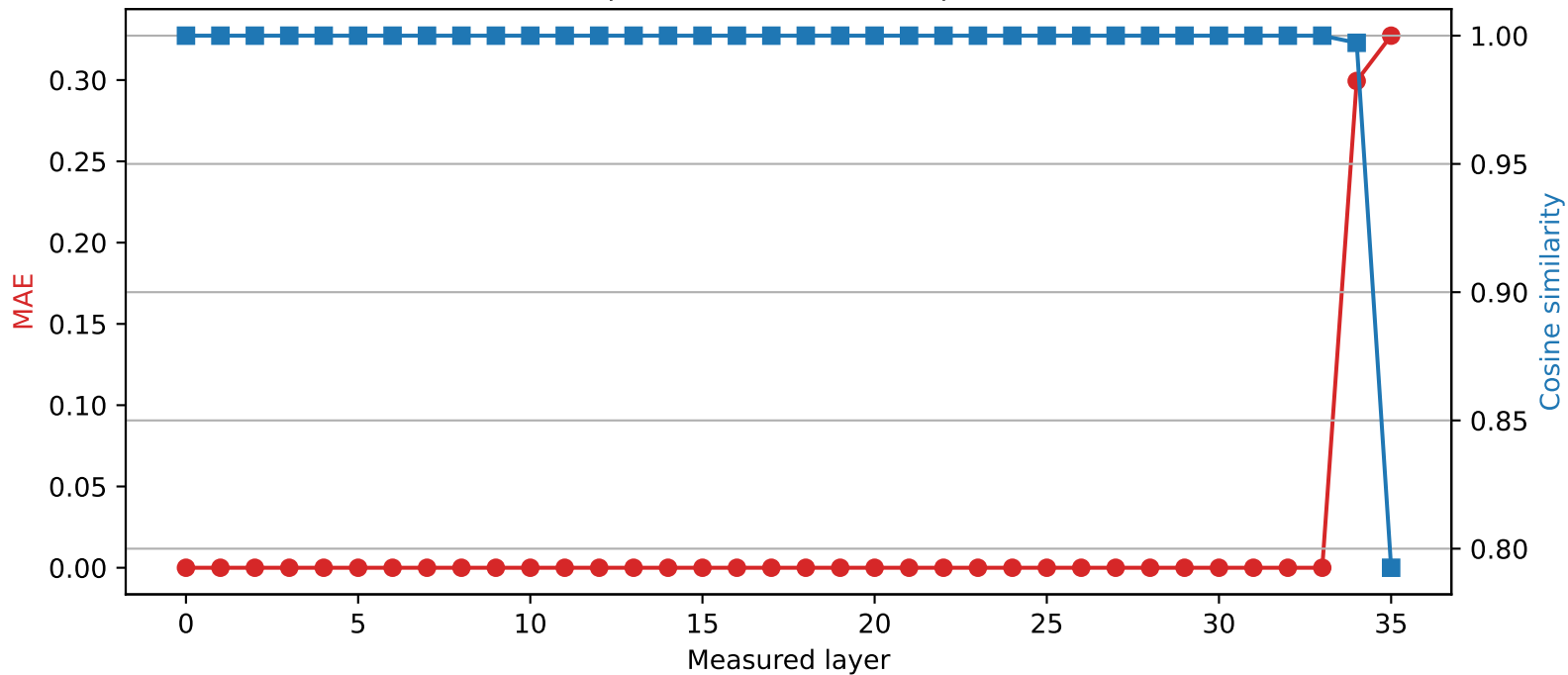
SmolLM3-3B | Quantized layer 33 | float64 \rightarrow int2
