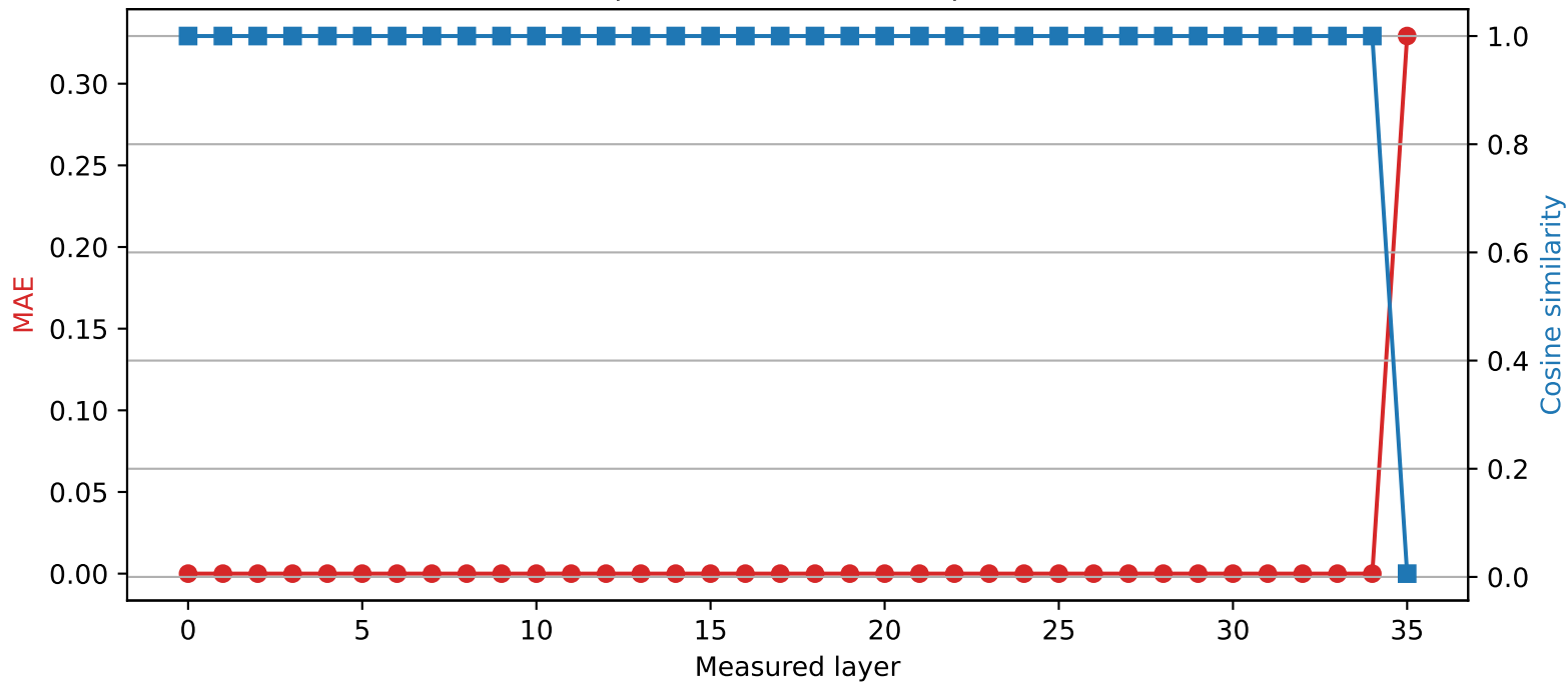
SmolLM3-3B | Quantized layer 34 | float64 \rightarrow int2
