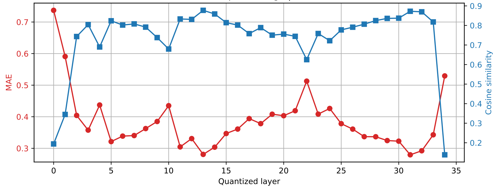
SmolLM3-3B | Prompt 1 Final RMSNorm output damage | float64 \rightarrow int2
