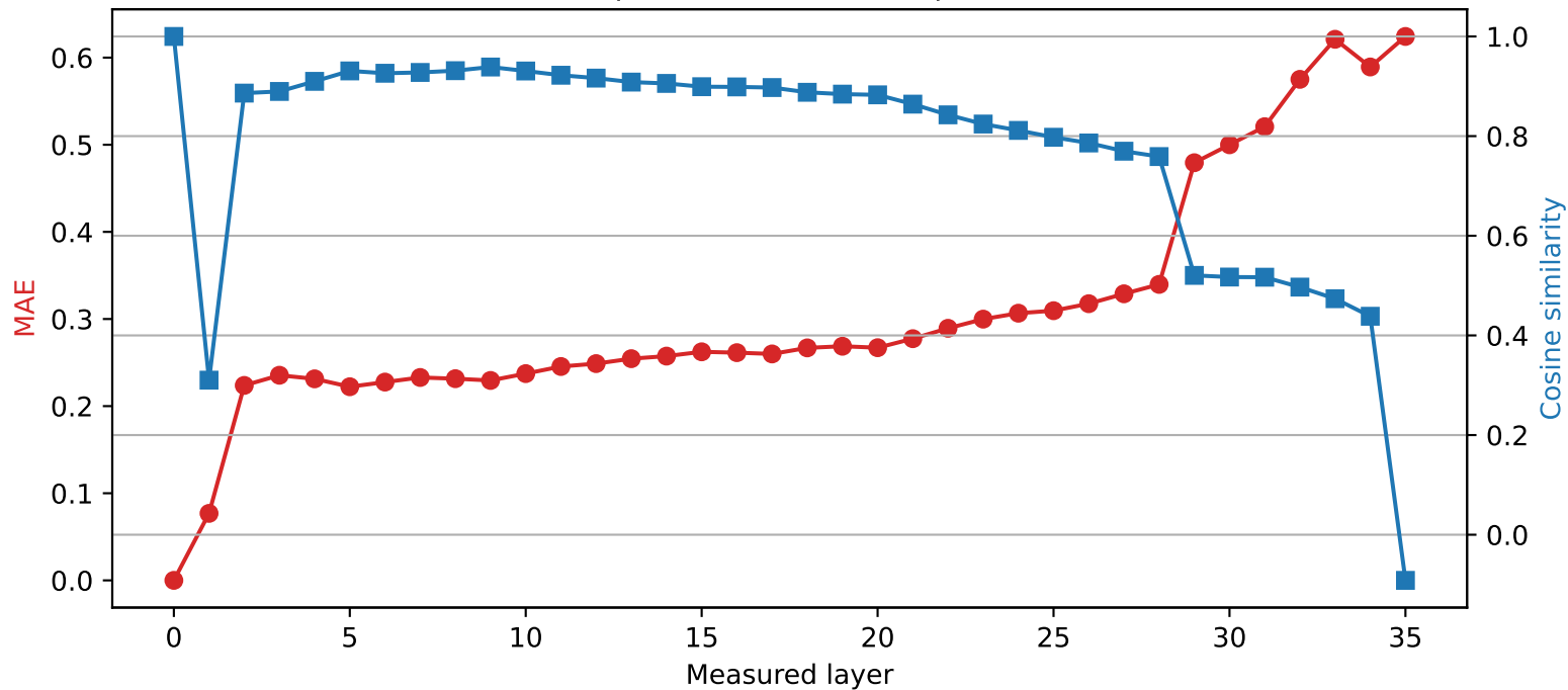
SmolLM3-3B | Quantized layer 0 | float64 \rightarrow int2
