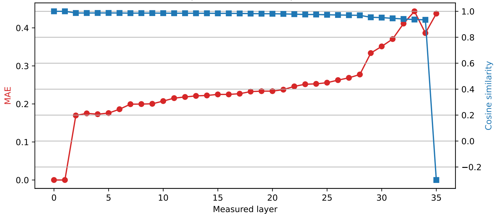
SmolLM3-3B | Quantized layer 1 | float64 → int2
