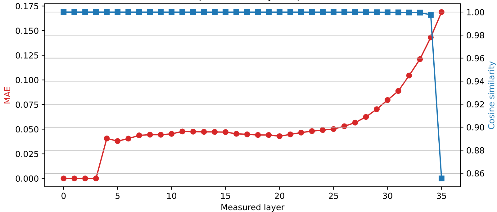
SmolLM3-3B | Quantized layer 3 | float64 → int2
