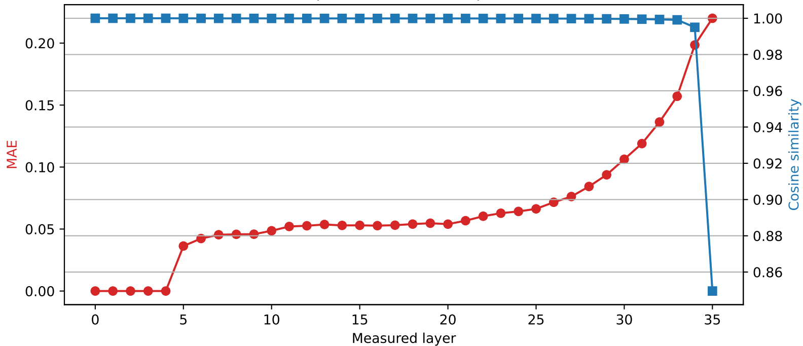
SmolLM3-3B | Quantized layer 4 | float64 → int2
