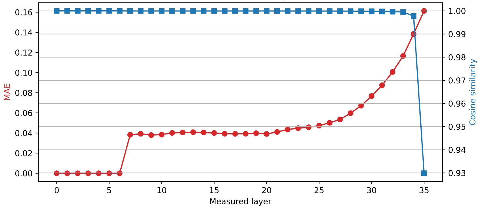
SmolLM3-3B | Quantized layer 6 | float64 \rightarrow int2
