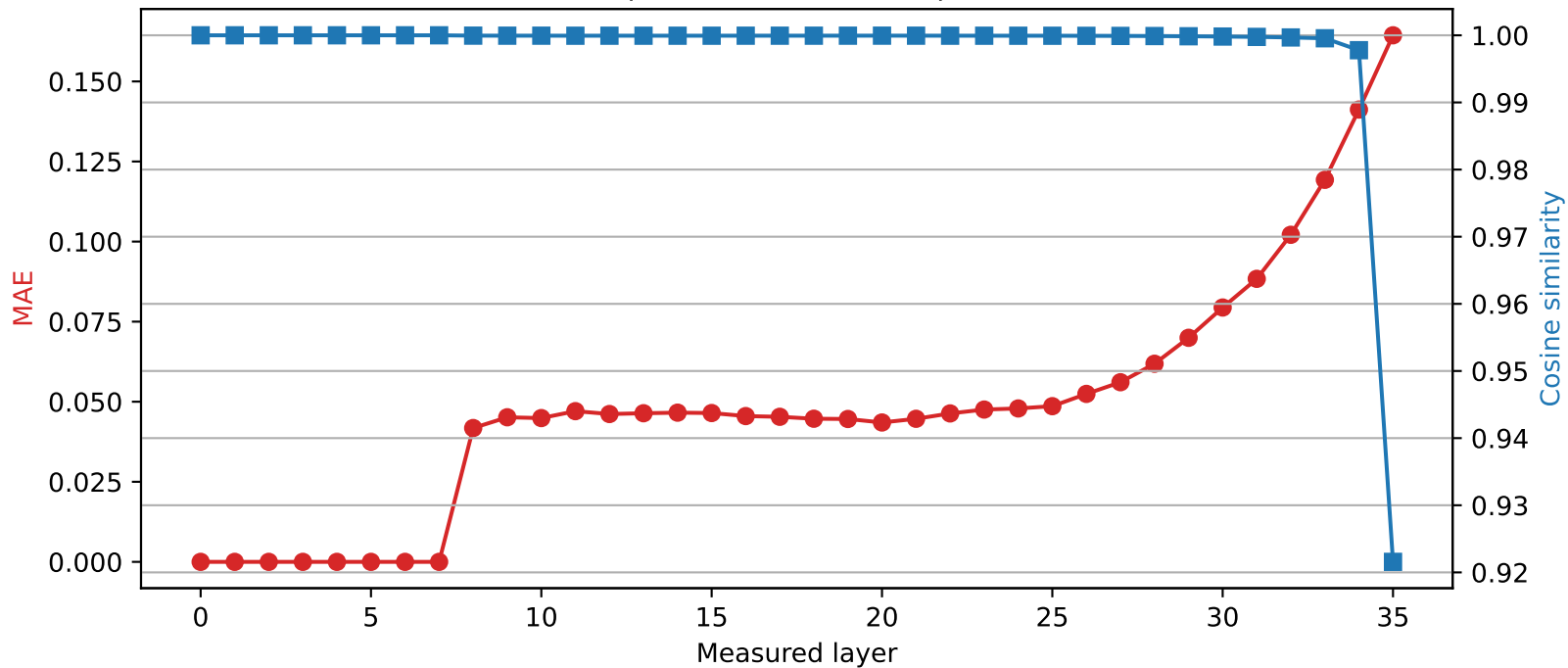
SmolLM3-3B | Quantized layer 7 | float64 \rightarrow int2
