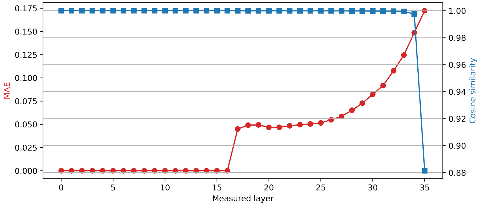
SmolLM3-3B | Quantized layer 16 | float64 \rightarrow int2
