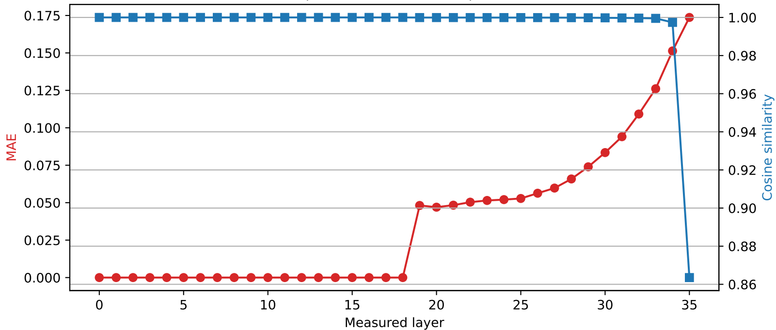
SmolLM3-3B | Quantized layer 18 | float64 → int2
