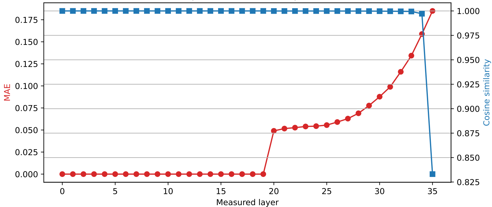
SmolLM3-3B | Quantized layer 19 | float64 → int2
