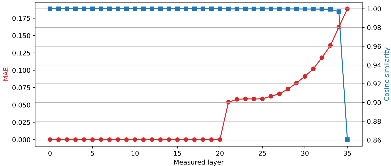
SmolLM3-3B | Quantized layer 20 | float64 \rightarrow int2
