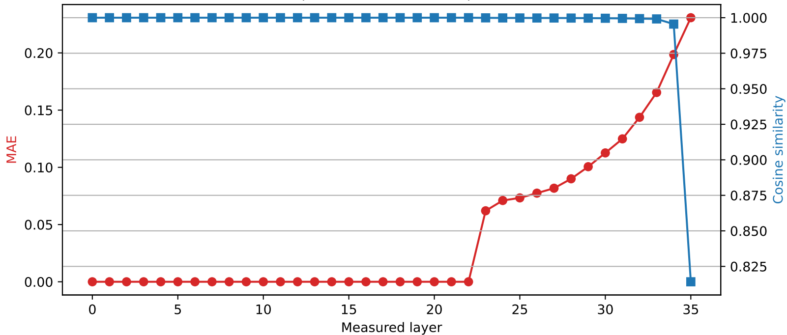
SmolLM3-3B | Quantized layer 22 | float64 \rightarrow int2
