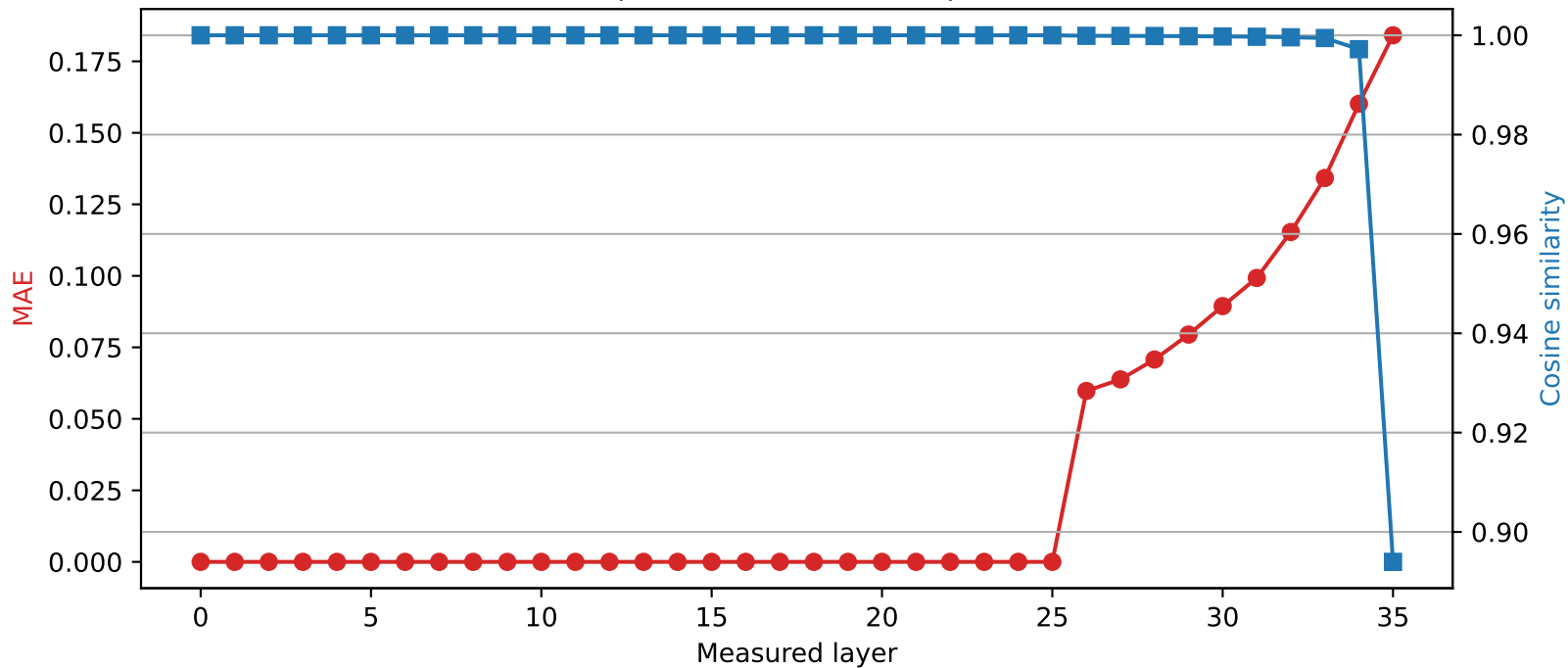
SmolLM3-3B | Quantized layer 25 | float64 \rightarrow int2
