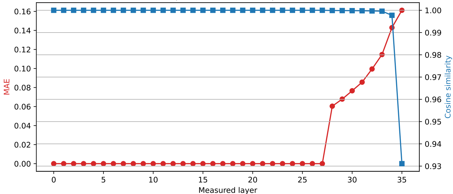
SmolLM3-3B | Quantized layer 27 | float64 \rightarrow int2
