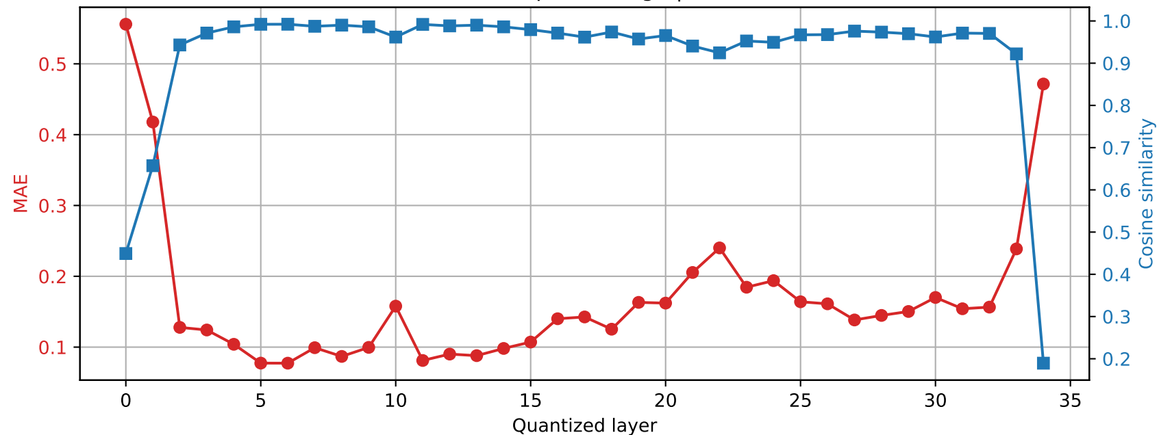
SmolLM3-3B | Prompt 2 Final RMSNorm output damage | float64 \rightarrow int2
